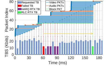
Fig. 19— RLC ReTXs inflate the packet delay by 105 ms, denoted as the yellow arrow.
