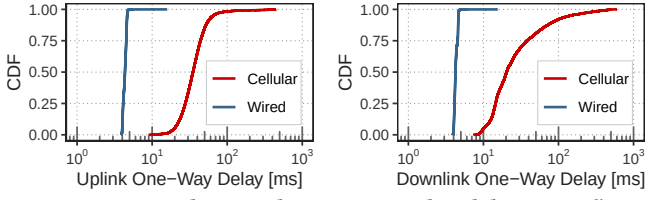
Fig. 2— 5G v. wired network one-way packet delay: 5G inflates median delay by 1-2 orders of magnitude.
