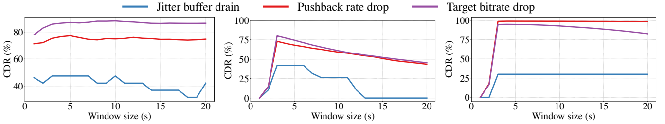
Fig. 12— Domino's performance of detecting cross traffic and channel degradation as the causes for different consequences across cells.
