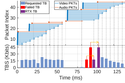
Fig. 18— HARQ ReTXs inflate the packet delay by 10 ms, denoted as yellow arrows.
